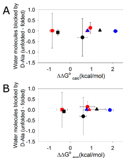
Figure 4. Changes in backbone solvation do not correlate with \Delta\Delta G^\circ . The difference in the number of water molecules blocked by D-Ala relative to Gly (unfolded–folded) is plotted vs (A) calculated \Delta\Delta G^\circ values ( r = 0.16 ). (B) experimental \Delta\Delta G^\circ values ( r = 0.17 ). EH, solid black circle; GA, solid red circle; HP35, solid red square; NTL9, solid blue circle; PSBD, solid black up triangle; Trp-cage, solid red up triangle; UBA, solid blue up triangle; ubiquitin, solid black square. Positive \Delta\Delta G^\circ values indicate stabilization.
