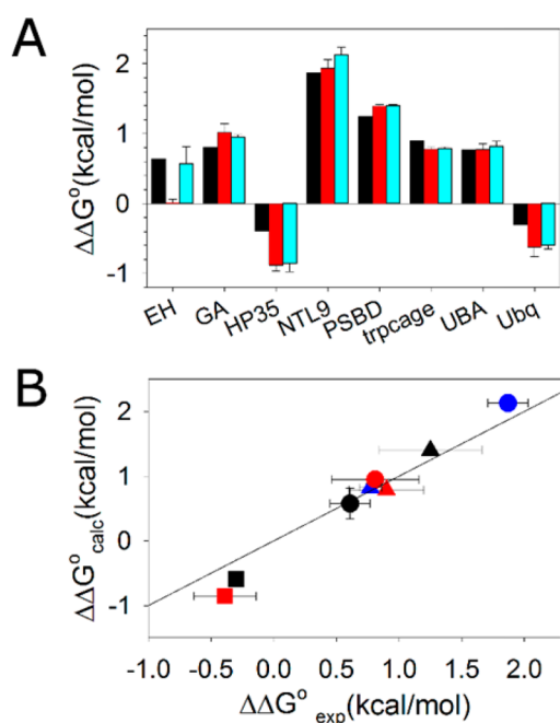
Figure 2. Thermodynamic integration reproduces experimental values of \Delta\Delta G^\circ . (A) Experimental \Delta\Delta G^\circ values are shown in black. Calculated \Delta\Delta G^\circ values using experimental structures as starting structures are shown in red. Calculated \Delta\Delta G^\circ values using the last frames of 50 ns simulations as the starting structures are in cyan. (B) Scatter plot of experimental \Delta\Delta G^\circ and calculated \Delta\Delta G^\circ values using the last frames of a 50 ns simulation as the starting structure. Solid line represents \Delta\Delta G^\circ_{\text{exp}} = \Delta\Delta G^\circ_{\text{calc}} . EH, solid black circle; GA, solid red circle; HP35, solid red square; NTL9, solid blue circle; PSBD, solid black up triangle; Trp-cage, solid red up triangle; UBA, solid blue up triangle; ubiquitin, solid black square. The calculated value for the EH domain used in the plot was derived by using the unrestrained MD structure as the starting structure for the TI calculation. Positive \Delta\Delta G^\circ values indicate stabilization.
