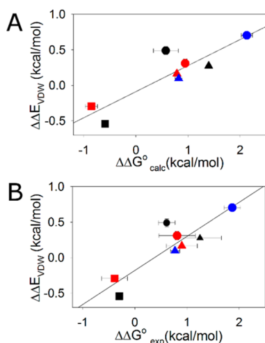
Figure 3. Scatter plot of \Delta\Delta E_{\text{vdw}} and \Delta\Delta G^\circ with solid line showing the linear fit. (A) Correlation of \Delta\Delta E_{\text{vdw}} and \Delta\Delta G^\circ values calculated by thermodynamic integration. r = 0.89 , p -value = 0.0033 (B) Correlation of \Delta\Delta E_{\text{vdw}} and experimental \Delta\Delta G^\circ values. r = 0.89 , p -value = 0.0033. EH, solid black circle; GA, solid red circle; HP35, solid red square; NTL9, solid blue circle; PSBD, solid black up triangle; Trp-cage, solid red up triangle; UBA, solid blue up triangle; ubiquitin, solid black square. Positive \Delta\Delta G^\circ values indicate stabilization.
