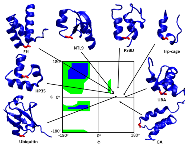
Figure 1. Ribbon representation of the proteins studied with the C-capping Gly colored red. \varphi/\psi angles of the C-capping glycines are indicated by arrows. The Ramachandran plot is colored green for broadly allowed and blue for most favored regions for L-amino acids, which is adopted from Ramaplot in VMD. 36 The Ramachandran plot for a D-amino acid is the mirror image about the central point ( \varphi = 0^\circ and \psi = 0^\circ ) of the plot shown above.
