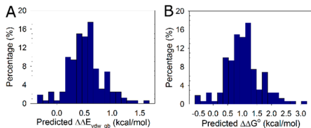
Figure 6. Proteins are stabilized by D-Ala substitutions. The distribution of \Delta\Delta E_{\text{vdw\_gb}} and \Delta\Delta G^{\circ} values for the 160 C-capping sites in the 120 nonredundant proteins is shown as a histogram. (A) Distribution of \Delta\Delta E_{\text{vdw\_gb}} values. (B) Distribution of predicted \Delta\Delta G^{\circ} values. Positive \Delta\Delta G^{\circ} values represent a stabilizing effect.
